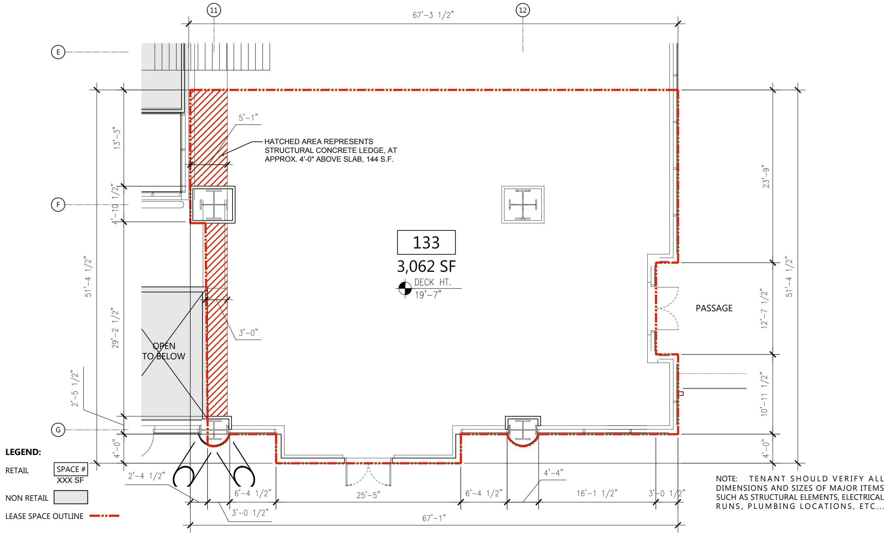
GROUND FLOOR PLAN, BLOCK "2"
